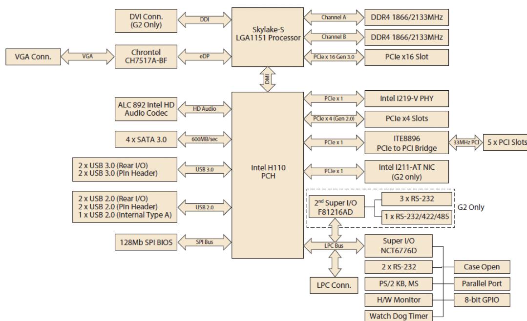
Figure 1.3 AIMB-705 Block Diagram
