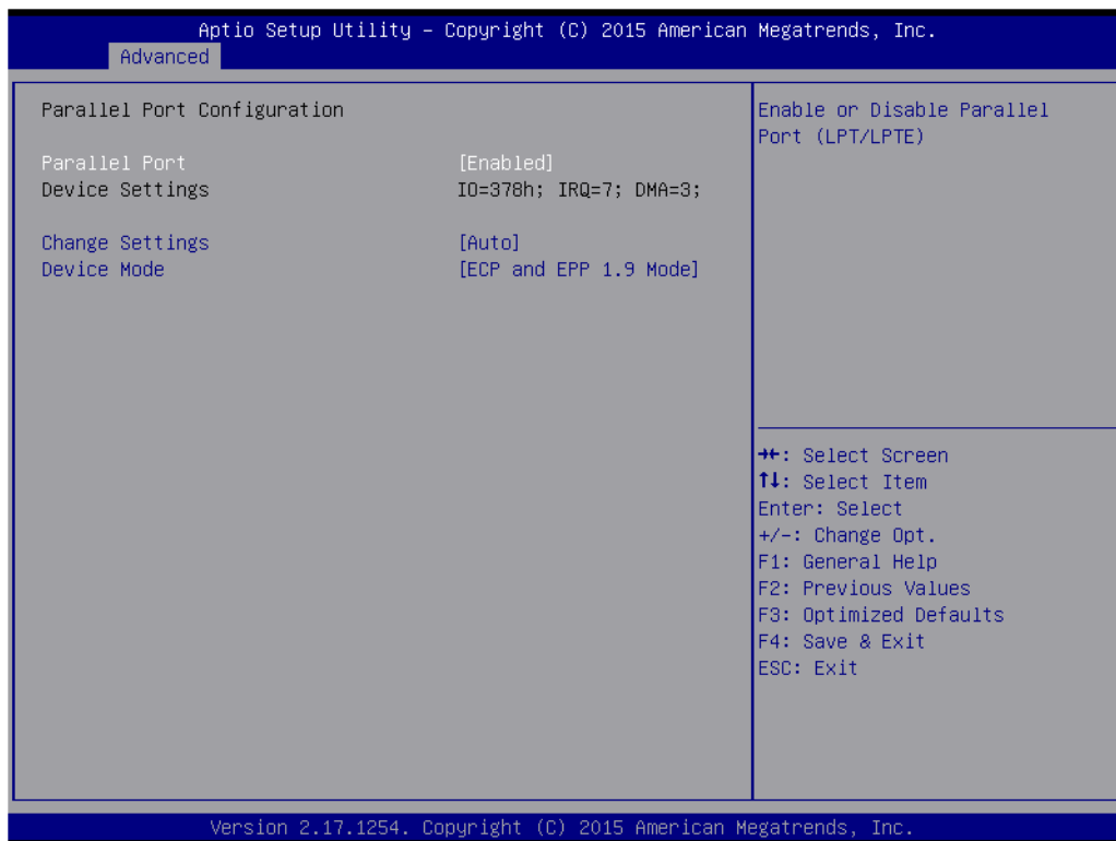
Figure 3.12 Parallel Configuration
