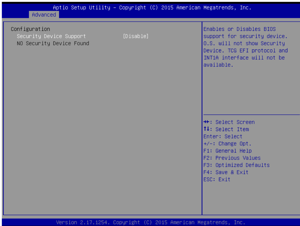
Figure 3.7 TPM Settings
