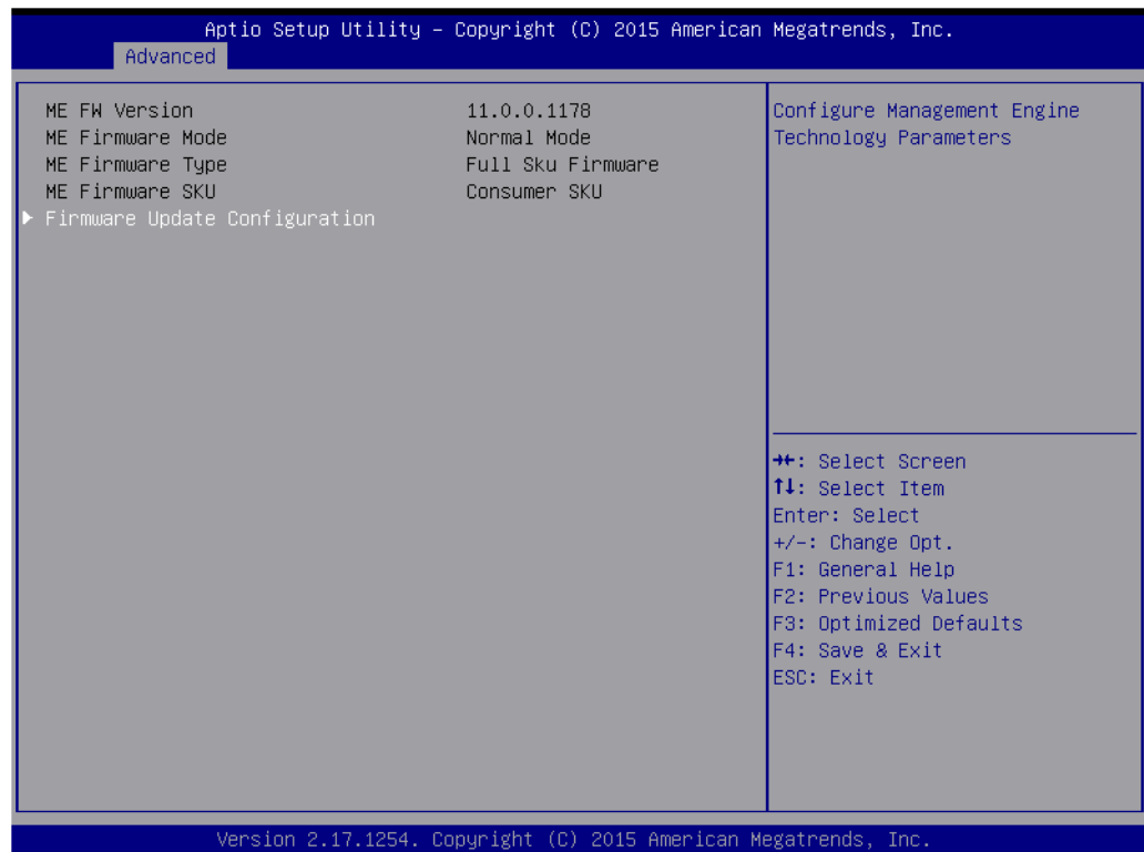
Figure 3.6 PCH-FW Configuration
