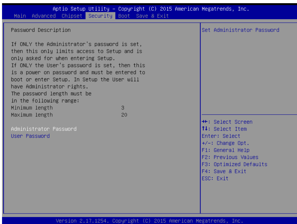
Figure 3.34 Security
